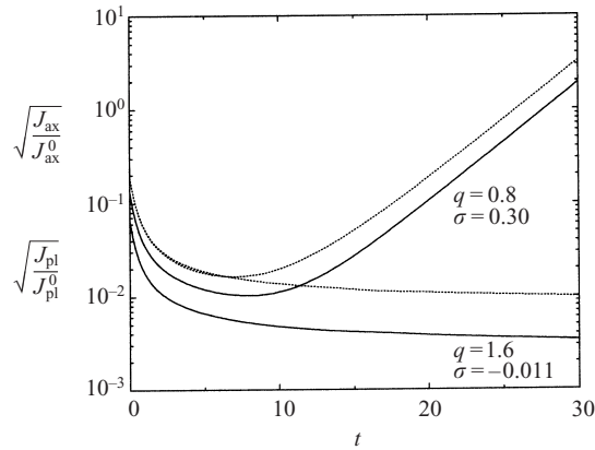
FIGURE 1. Temporal evolution of (J_{\text{pl}}/J_{\text{pl}}^0)^{1/2} (solid line) and (J_{\text{ax}}/J_{\text{ax}}^0)^{1/2} (dotted line) for \gamma = 0 at swirl numbers q = 0.8 and q = 1.6 , with Re = 667 .
