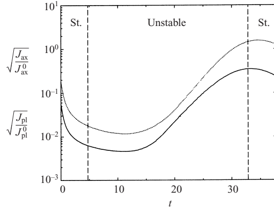
FIGURE 5. Temporal evolution of quantities (J_{pl}/J_{pl}^0)^{1/2} (solid line) and (J_{ax}/J_{ax}^0)^{1/2} (dotted line) for the simulation with compression and stretching. The dashed line corresponds to the Batchelor-vortex instability threshold.
