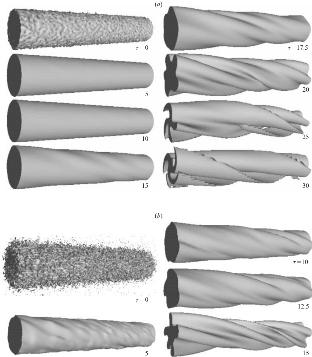
FIGURE 10. Isosurfaces of the axial component \Omega_z of the total vorticity for \Omega_z(\bar{r}, \theta, \bar{z}, \tau) = \frac{1}{2}\Omega_{z,\max} . For series (a), the simulation is initiated with a r.m.s. value (J_{\text{pl}}(0)/J_{\text{pl}}^0)^{1/2} = 8 \times 10^{-4} . For series (b), a stronger noise amplitude is used (J_{\text{pl}}(0)/J_{\text{pl}}^0)^{1/2} = 1.4 \times 10^{-2} . Each snapshot corresponds to a circle in figures 3 and 4. Note that the conical aspect of the vortex is only due to the geometrical perspective.
