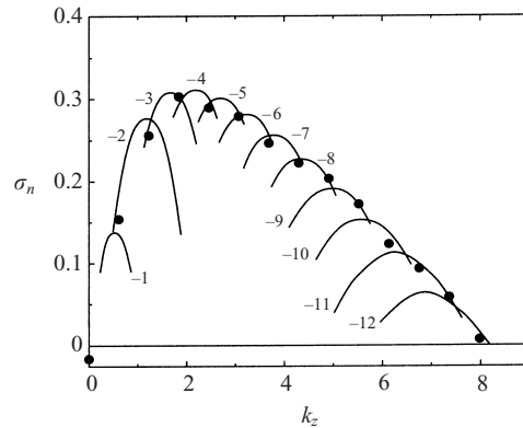
FIGURE 2. Temporal growth rate \sigma as a function of axial wavenumber k_z for parameters \gamma = 0 , q = 0.8 and Re = 667 . The symbols \bullet denote the growth rates of the discrete axial wavenumbers obtained in the present simulation, computed from the time evolution of perturbation spectra. Each solid line (reported from Delbende et al. 1998) shows the growth rate \sigma_n(k_z) for each unstable azimuthal wavenumber n ( n is indicated near the associated curve) obtained from a viscous DNS-based stability analysis at the same Reynolds number.
