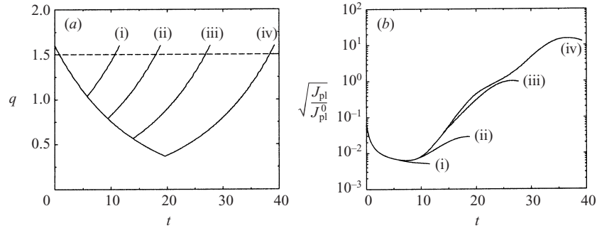
FIGURE 11. Various simulations (i–iv) with compression and stretching for the same value of \tilde{\gamma} = \pm 0.05 and for various time intervals T_{\text{inst}} . (a) Instantaneous swirl number q(t) ; (b) temporal evolution of energy (J_{\text{pl}}/J_{\text{pl}}^0)^{1/2} .
