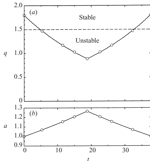
FIGURE 4. Instantaneous (a) swirl number q(t) and (b) core size a(t) as functions of physical time t for the simulation with compression and stretching. The dashed line corresponds to the Batchelor-vortex instability threshold at q \approx 1.50 . The circles denote the position of the snapshots pictured in figures 6–10.
