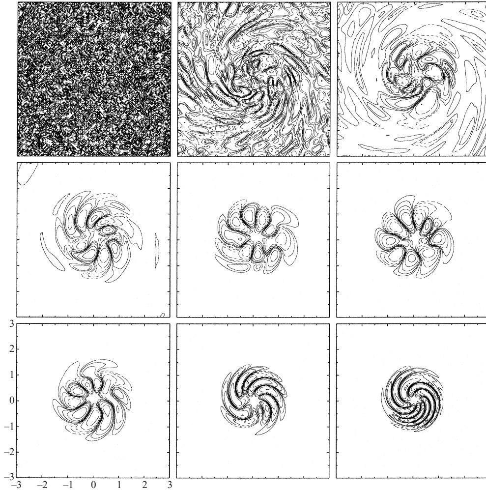
FIGURE 8. Isocontours in the (r, \theta) -plane of the axial component \omega_z of the perturbation vorticity at a fixed axial location. Contours shown correspond to \omega_z(r, \theta, t) = \pm \omega_{z,\max}/2^p , where p = 1, 2, \dots, 5 . Positive (resp. negative) values are represented by solid (resp. dashed) lines. Each snapshot corresponds to a circle in figures 3 and 4. Figure should be read from left to right and top to bottom.
