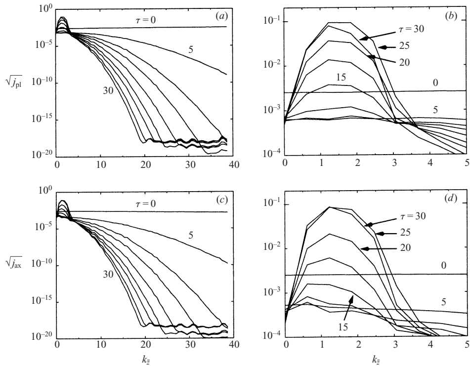
FIGURE 6. Spectrum of transverse j_{pl}^{1/2} (a, b) and axial j_{ax}^{1/2} (c, d) r.m.s. perturbation velocities with respect to the axial wavenumber k_z at \tau = 0, 5, 10, 12.5, 15, 17.5, 20, 25, 30 . Frames (b) and (d) are close-ups of the low-wavenumber region, where pertinent phenomena occur.
