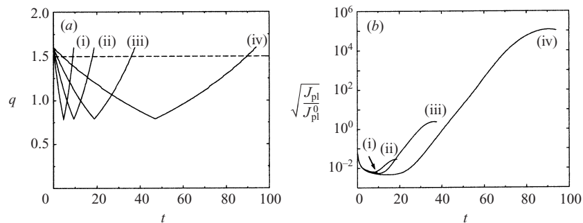
FIGURE 12. Various simulations (i–iv) with compression and stretching for different values of \tilde{\gamma} (respectively \pm 0.1 , \pm 0.05 , \pm 0.025 , \pm 0.01 ). (a) Instantaneous swirl number q(t) ; (b) temporal evolution of energy (J_{\text{pl}}/J_{\text{pl}}^0)^{1/2} .
