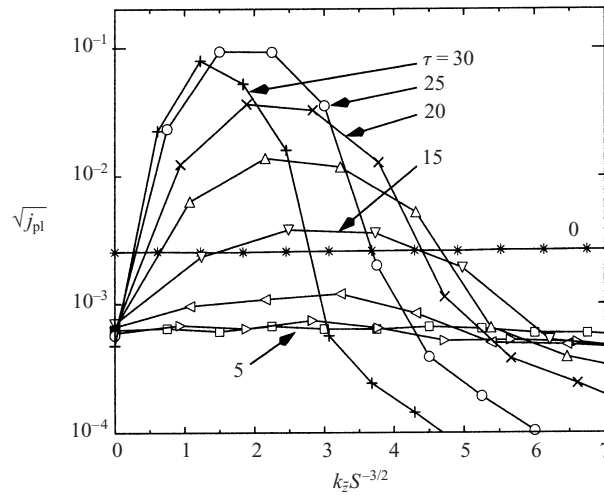
FIGURE 7. Same as figure 6(b) but plotted with respect to the rescaled wavenumber k_z S^{-3/2} .
