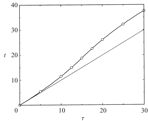
FIGURE 3. Physical time t versus modified time \tau used for the simulation with compression and stretching. The circles denote the position of the snapshots pictured in figures 6–10. The straight line indicates function t = \tau prevailing when \gamma = 0 .
