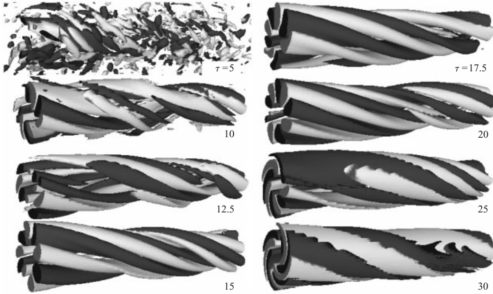
FIGURE 9. Isosurfaces of the axial component \omega_z of the perturbation vorticity for \omega_z(\bar{r}, \theta, \bar{z}, \tau) = \pm \frac{1}{2} \omega_{z,\max} . Each snapshot corresponds to a circle in figures 3 and 4. Note that the conical aspect of the vortex is only due to the geometrical perspective.
