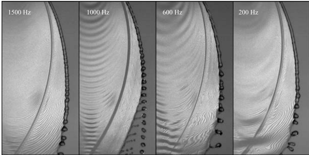
FIGURE 13. Effect of vibrations of the experimental structure on the thickness field and rim destabilization for different excitation frequencies, d_j = 1.05 \text{ mm} , u_j = 3.5 \text{ m s}^{-1} , 2\alpha = 90^\circ .
