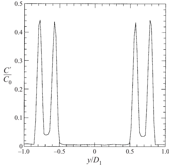
FIGURE 3. Radial profile of the r.m.s. fluctuations of concentration at x/e = 3 , Re = 1400 .
