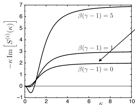
Arrhenius law with \beta_N q_N = 0.1
