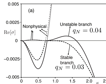
(\gamma - 1) = 0.1, \beta_N = 10, M_u^2 = 50
