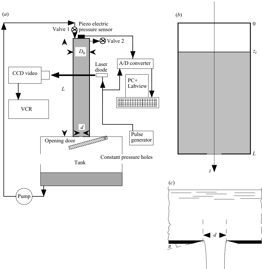
FIGURE 3. Experimental set-up: (a) general principle of the apparatus, (b) schema and orientation of axes, (c) close-up view of the hole.
