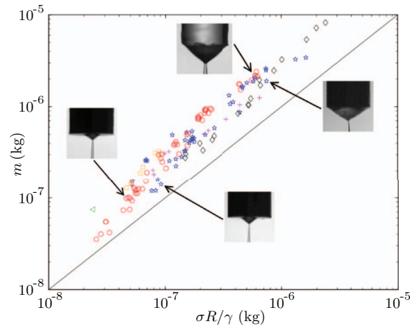
FIG. 4. Extracted mass as a function of \sigma R/\gamma (in kg). The solid line is the scaling in Eq. (2) and the symbols are the same as in Fig. 3. The four insets correspond to the last instant before breakup, for: (left) ethanol, R = 1.5 mm, \gamma = 66 g; (top) ethanol, R = 1.5 mm, \gamma = 4 g; (right) water, R = 1.5 mm, \gamma = 11 g; (bottom) water, R = 1.5 mm, \gamma = 112 g.
