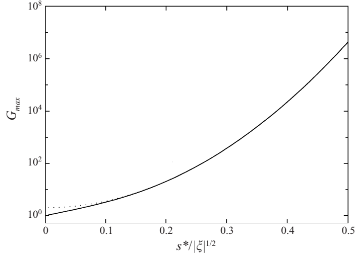
FIGURE 5. Plot of the maximum gain G_{max} as a function of s^*/|\xi|^{1/2} for the smallest resonant wavenumber \kappa \approx 1.13 . Solid line: G_{max} = (g_1 + g_2)^{1/2} , dotted line: 2 \exp(s^*/s_c^*)^2 .
