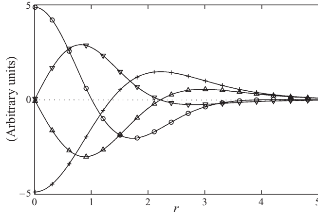
FIGURE 3. Four components of the eigenvector \Phi^+(r) = (iu_r, u_\theta, u_z, p) for \kappa = 1.13 : + , u_r ; o , u_\theta ; \Delta , u_z ; \nabla , 30 \times p .
