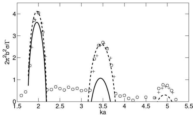
FIG. 1. Comparison of the growth rate computed with the two codes for \text{Re}=14\,000 and a/b=0.14 . Circles and crosses are data obtained with the fully spectral code and with the spectral-element code, respectively. Theoretical predictions are in solid line [formula (6.1a) from Le Dizès and Laporte (Ref. 7)] and in dashed line [same formula with a viscous damping term computed by the global approach (see text)].
