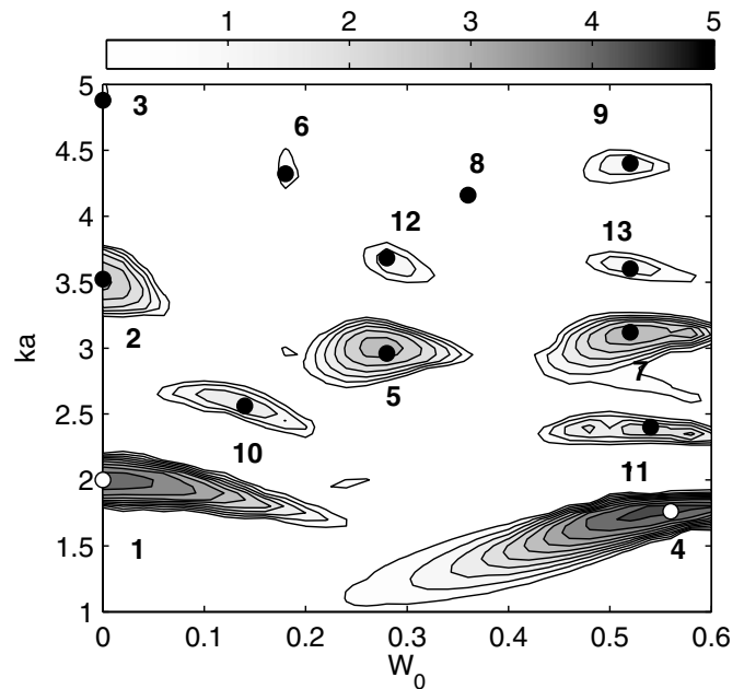
FIG. 2. Contours of instability growth rate in the (W_0, ka) plane for a/b=0.14 and \text{Re}=14\,000 . A number has been provided to each important unstable mode and is used hereafter to refer to each of them.
